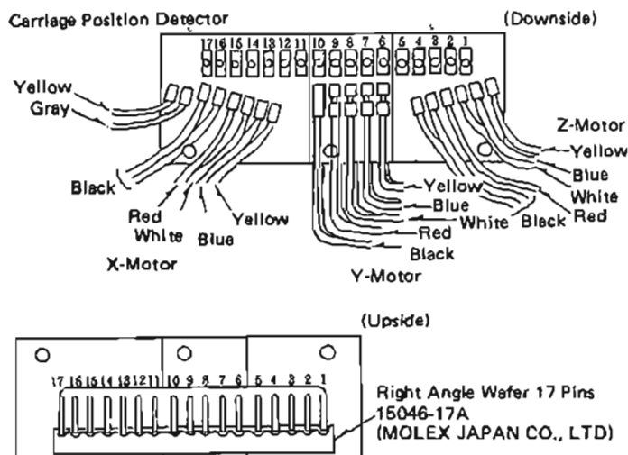
Figure VII-1: Wiring Diagram
