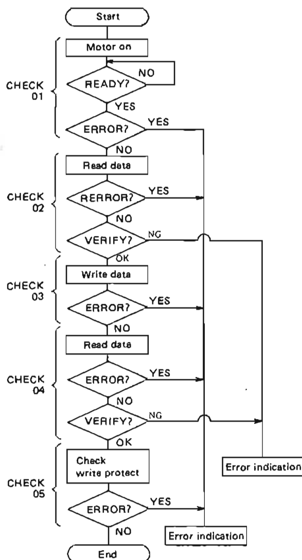
Test flowchart
