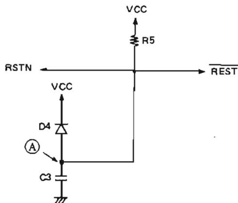
Fig. 1 Reset circuit
