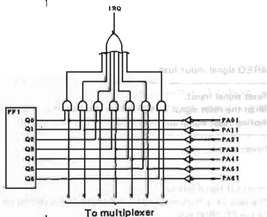
(Fig. 3) Interrupt circuit
