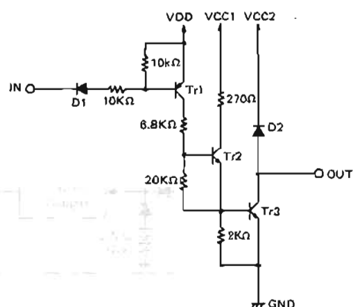
(Fig.7) Driver (LB1247) equivalent circuit
