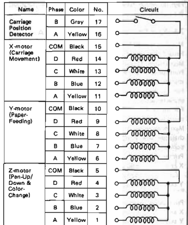
Figure VII-2: Circuit Diagram
