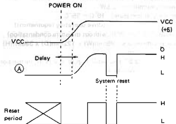
Fig. 2 Reset timings
