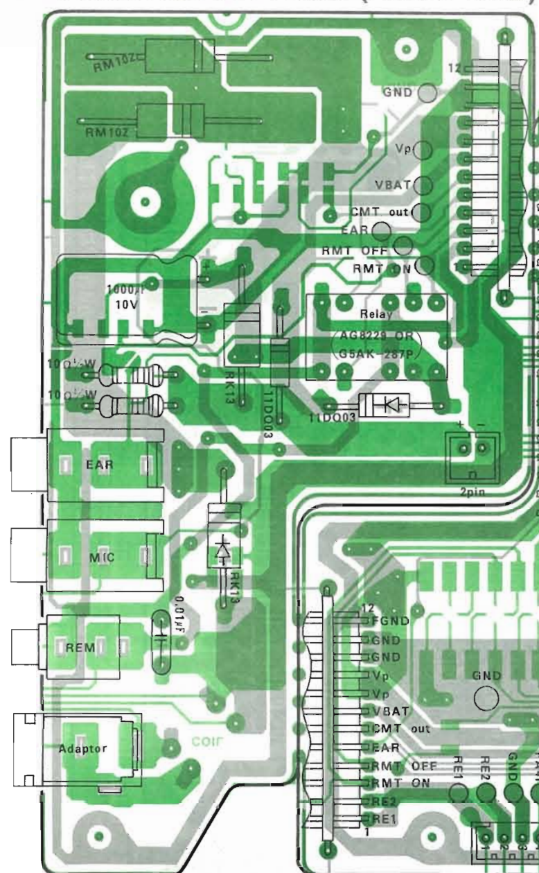
POWER SUPPLY P.W.B. (FRONT VIEW)
