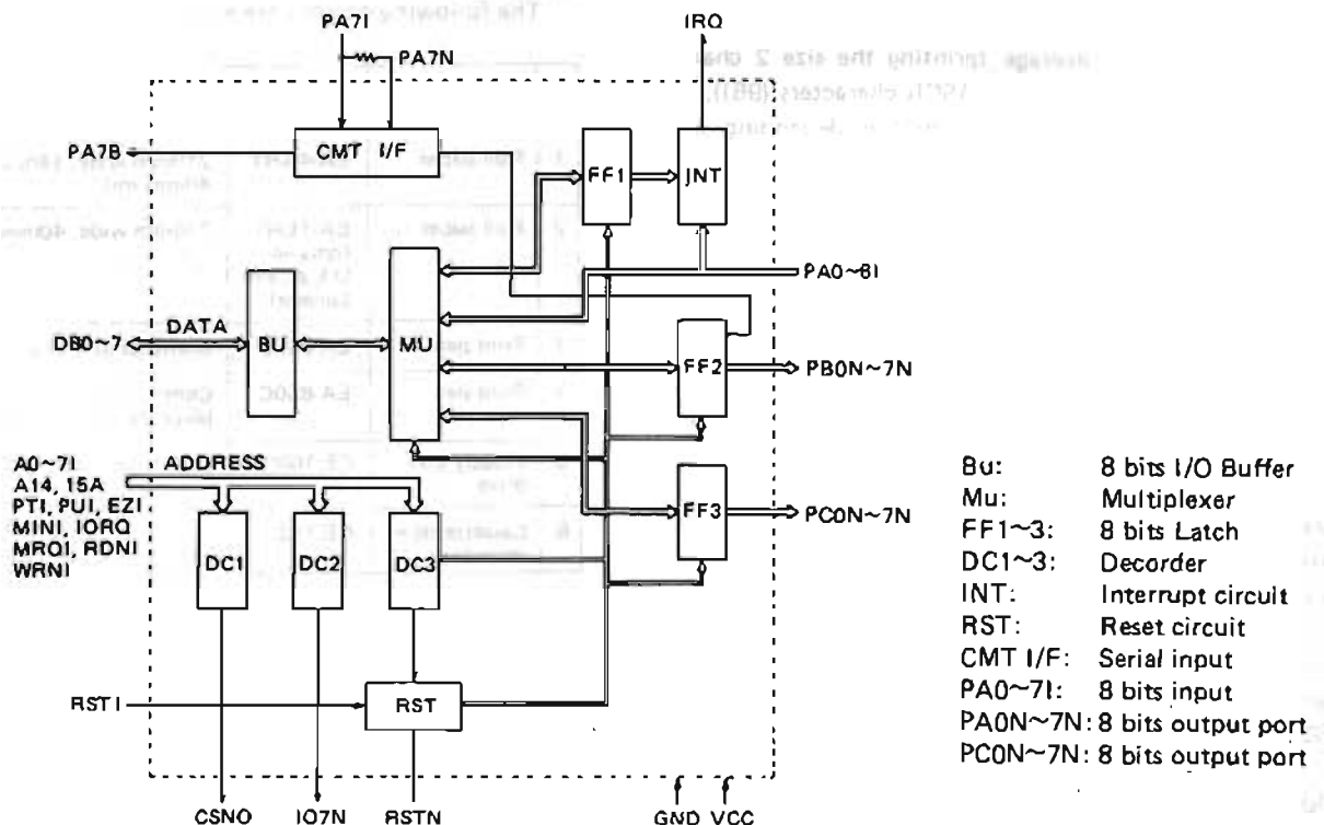
(Fig.1) LR38045 gate array block diagram
